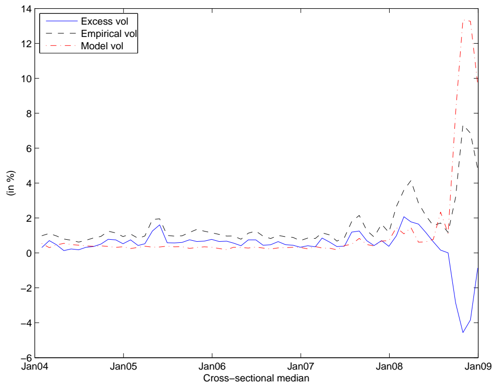
Figure 1: Time-series of empirical and model volatilities for synthetic floating rate bonds. The top panel is the cross-sectional mean for each period and the bottom panel is the cross-sectional median.
